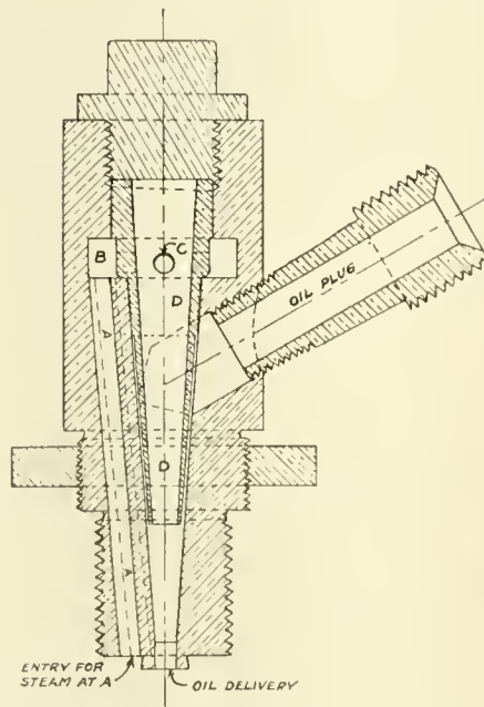
POSITIVE OIL DELIVERY DEVICE.
